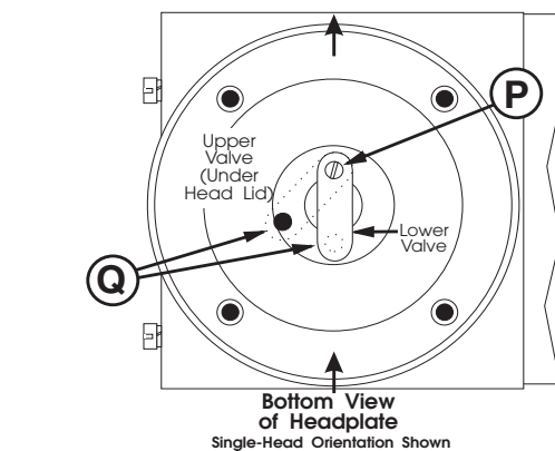
Valve Installation
